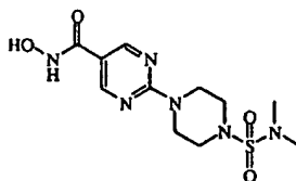
compound 2
